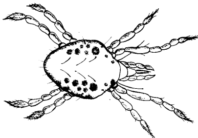
Figure 13: Mite (0.1 - 0.8 mm)
