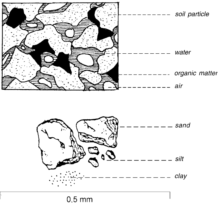
Figure 11: The proportions of solid particles, organic matter, water and air in the soil (Hillel, 1980 and Barbera Oranje).
