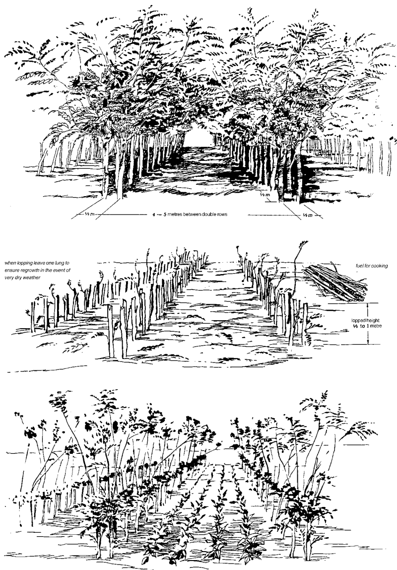
Figure 5: Alley cropping (Source: Wijewardena & Waidyanatha, 1984).
