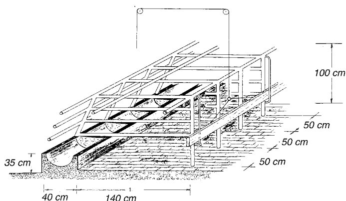
Figure 7: Separate feeding for pigs (from: Udo, 1985).
